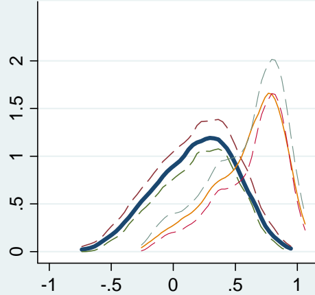
Distribution 1980M1-1983M12
