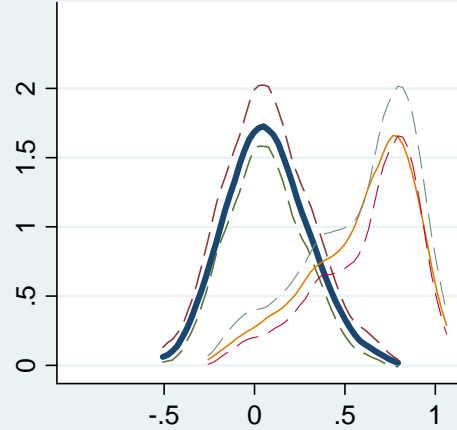
Distribution 1984M1-1988M12
