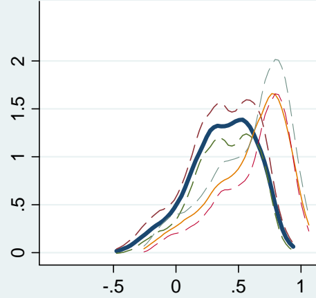
Distribution 1999M1-2003M12
