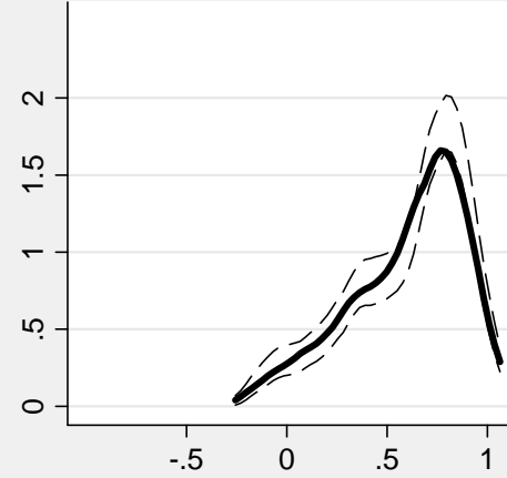
Distribution 2004M1-2009M4
