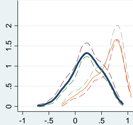
Distribution 1989M1-1993M12
