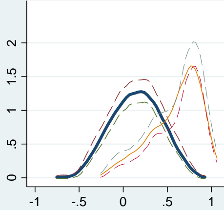
Distribution 1994M1-1998M12
