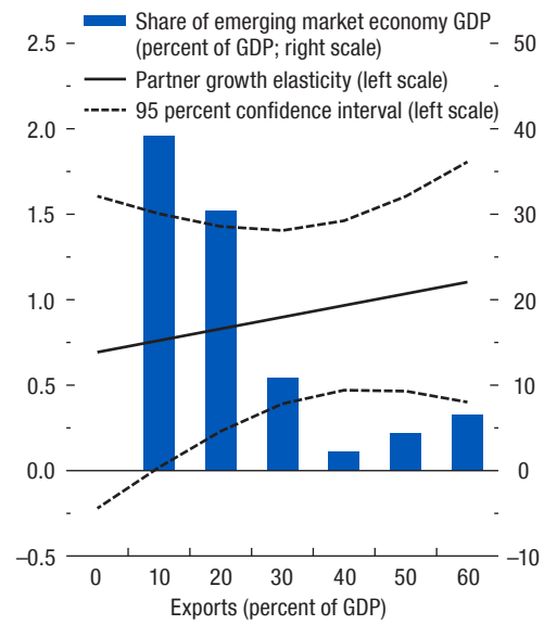
Figure 4.1.1. Export Partner Growth Elasticity
