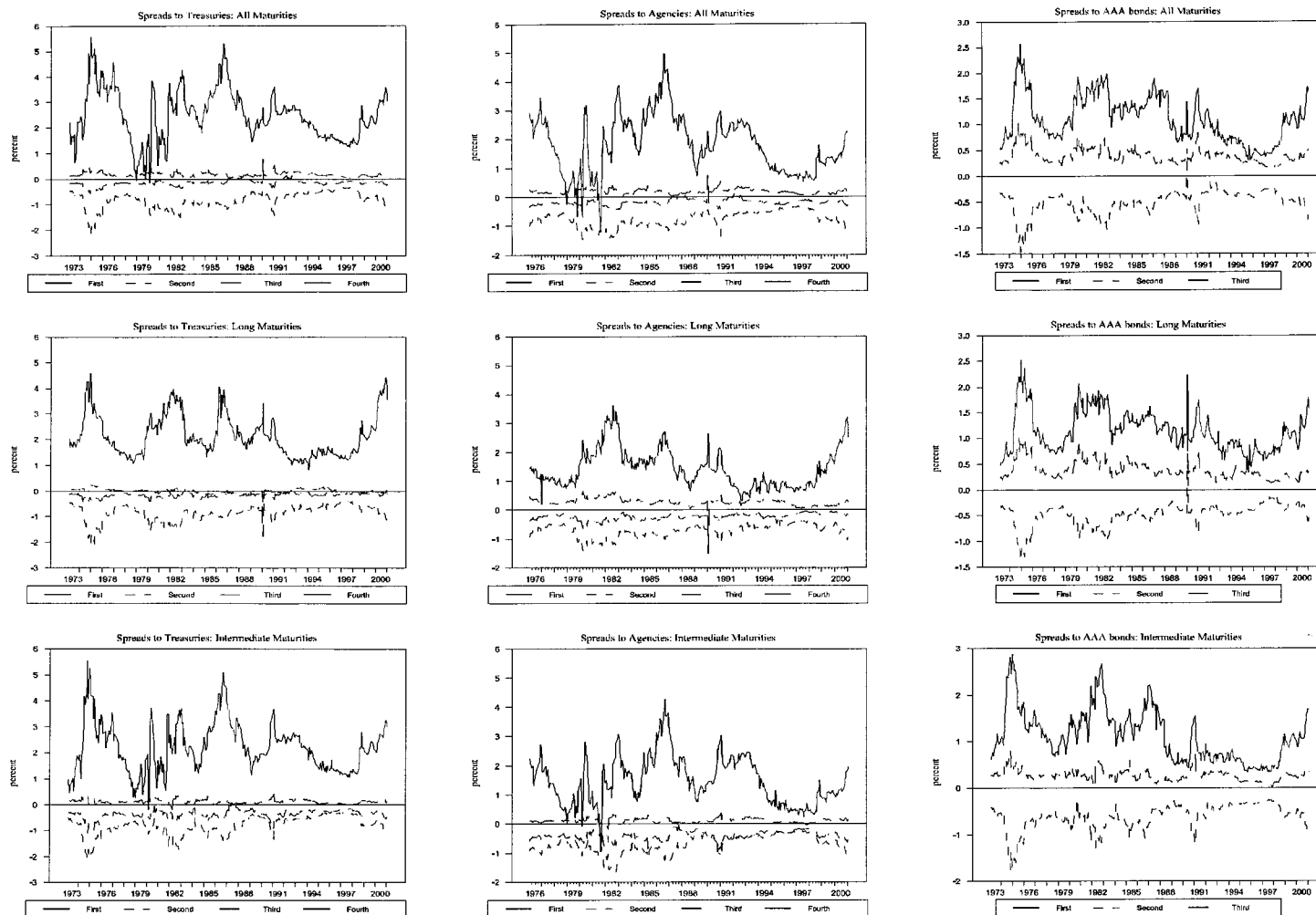
Figure 5: Principal Components of Credit Spreads
