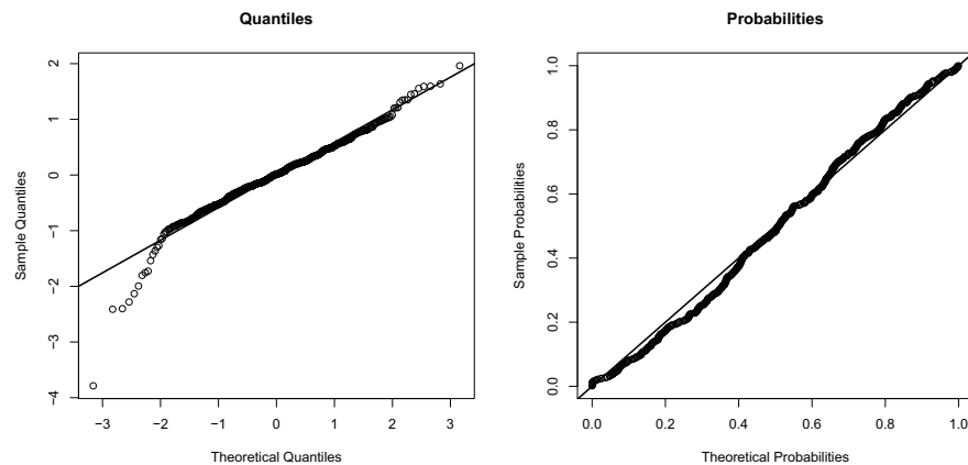
Figure 2: Plots for normality of residuals from model (3a)
