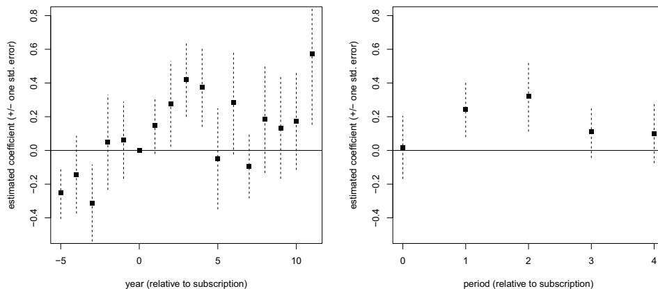
Figure 4: Dynamic effects of SDDS subscription
