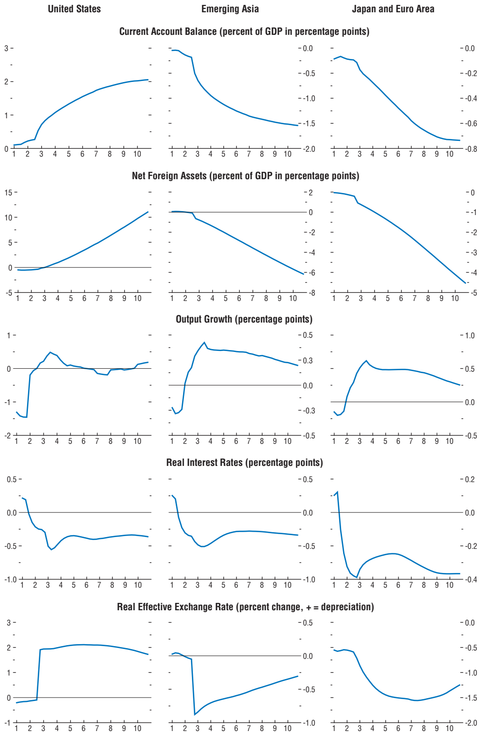
Figure 1.33. Incremental Effects of Fiscal Consolidation in the United States (Deviation from baseline; x-axis in calendar years)
