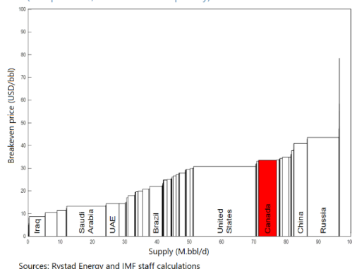
Canada: Global Oil Supply Cost Curve (USD per Barrel, Millions of Barrels per Day)
