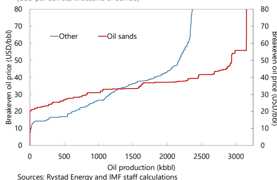
Canada: Oil Supply Cost Curve (USD per barrels, thousand of barrels)
