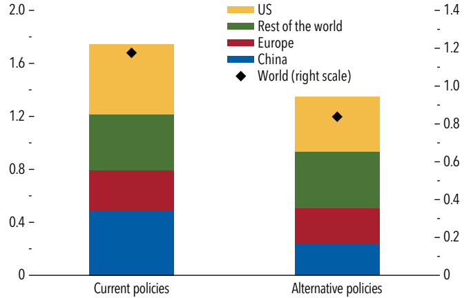
Figure 1.SF.5. Emission Impacts of Expansion in IT Sector (MtCO 2e ; cumulative greenhouse gas emissions; Percent change relative to that in baseline, right scale)
