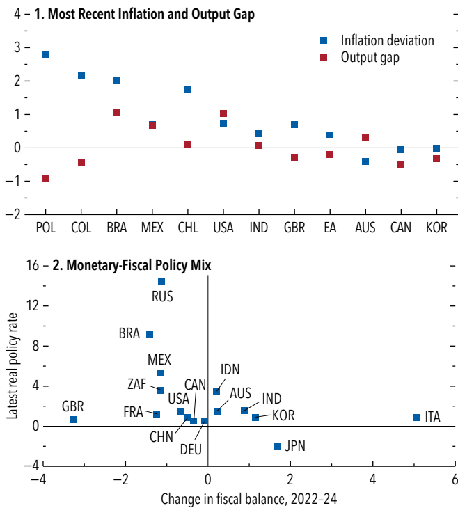
Figure 1.6. Cyclical Positions (Percent)
