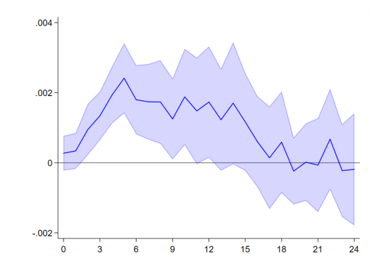
(f) Double-clustered standard errors
