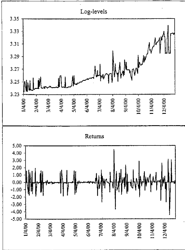
Figure 5: Mauritius: Log Levels and Returns (Jan 3 - Dec 29, 2000)
