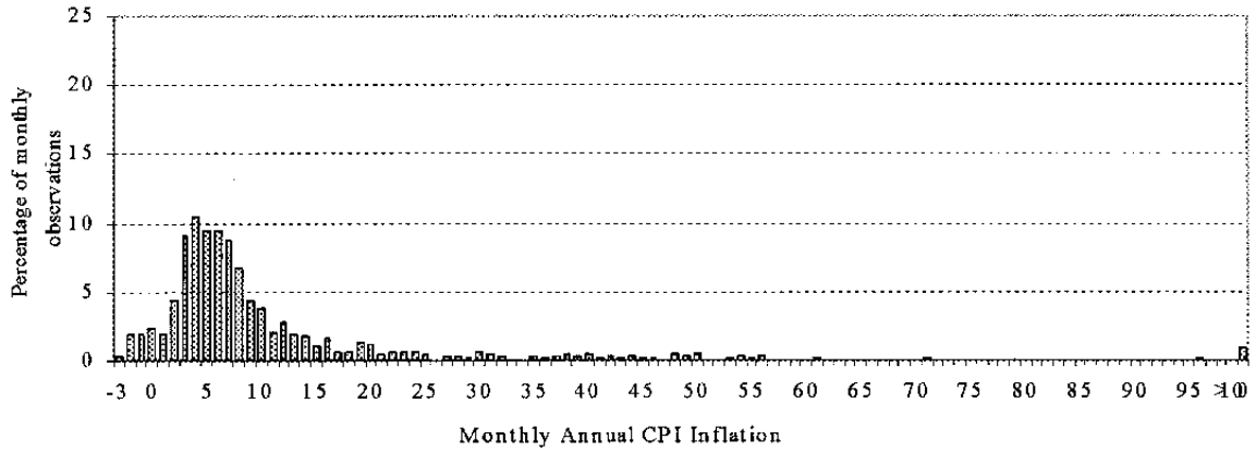
Figure 1a. IFL Countries: Year over Year Monthly CPI Inflation Density January 1999-May 2002
