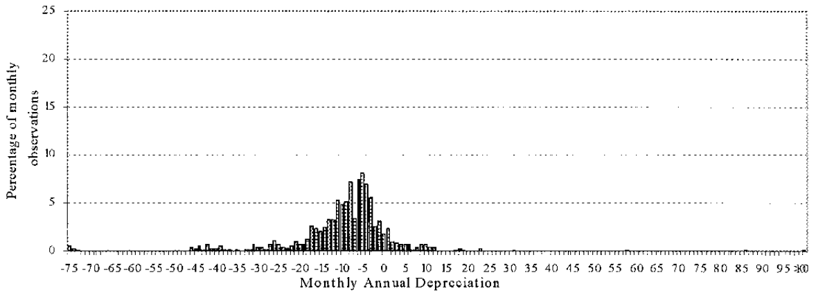
Figure 2a. IFL Countries: Year over Year Monthly Exchange Rate Change Density January 1999-May 2002
