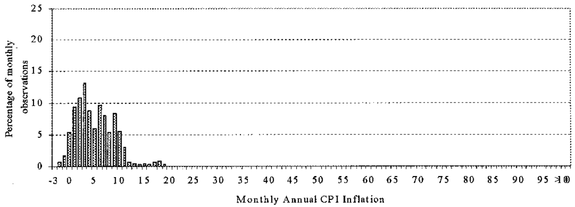
Figure 1b. FFIT Countries: Year over Year Monthly CPI Inflation Density January 1999-May 2002
