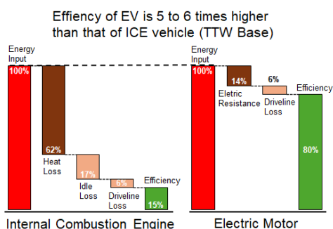
Figure 12. Relative Efficiency of Electric Vehicles (EVs) vs. Internal Combustion Engine (ICE) Vehicles
