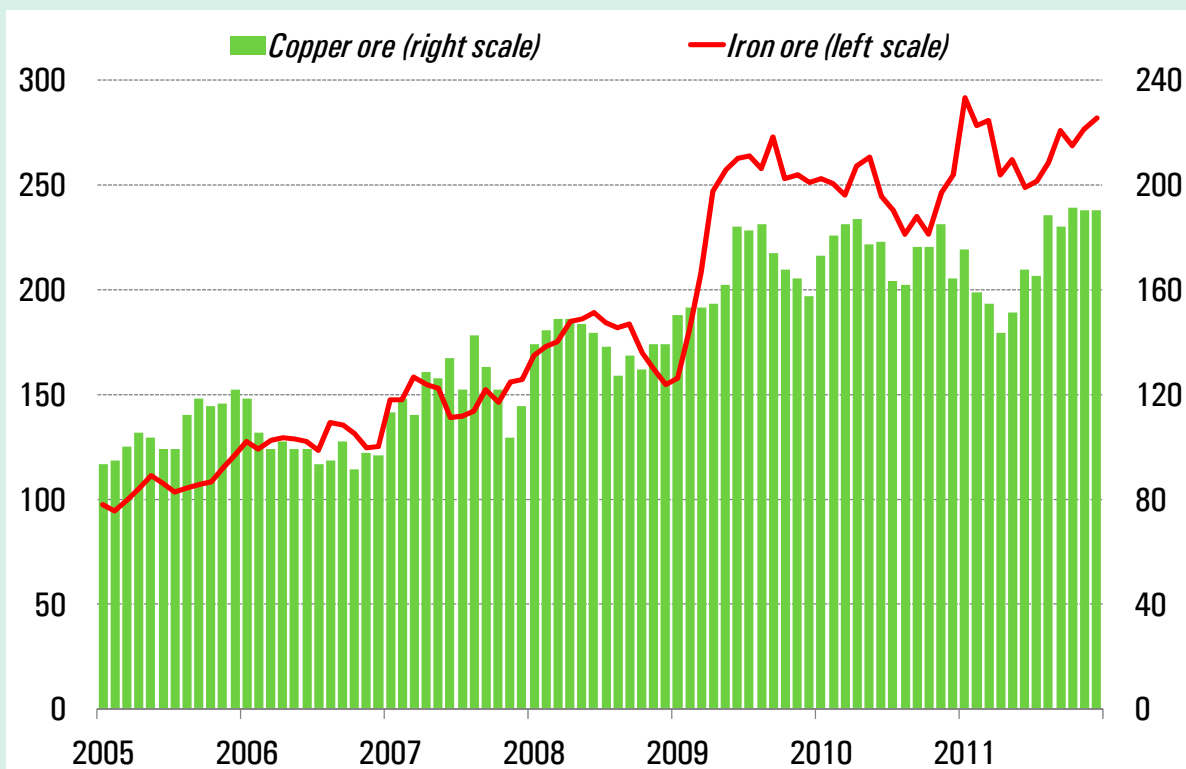
Figure 4.4. China: Mineral Import Volumes (Index, 2005:Q1 = 100, three-month moving average)
