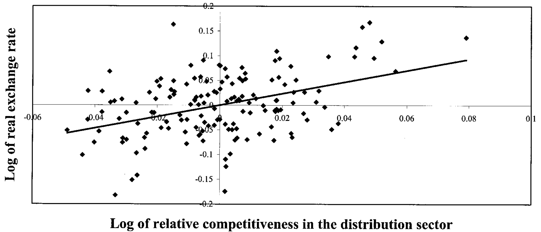
Figure 2. Conditional correlation
