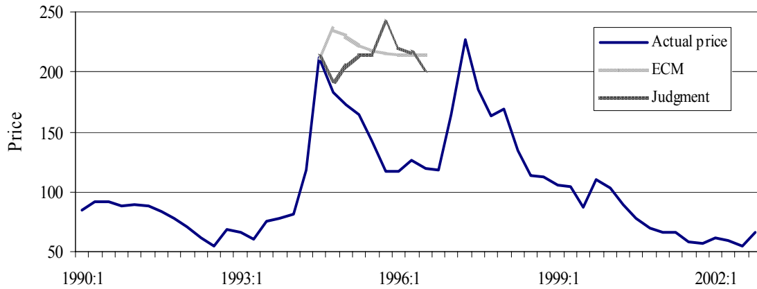
Figure 4. Coffee (Other Milds): Judgmental and ECM Forecasts, 1994: Q3
