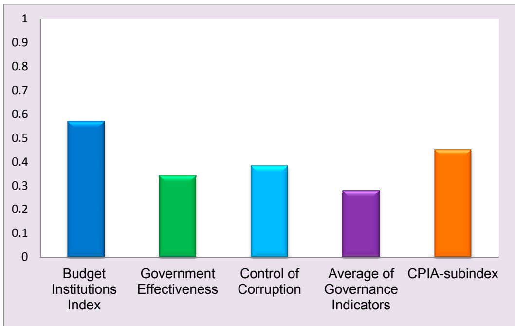
Figure 3. Spearman Correlation Between PIMI and other Indices
