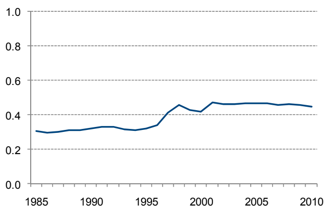
Figure 5. Time-varying PIMI (normalized)
