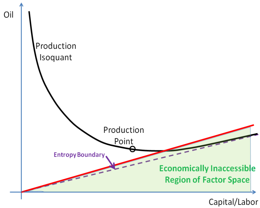
Figure 2. The Entropy Boundary in Factor Space
