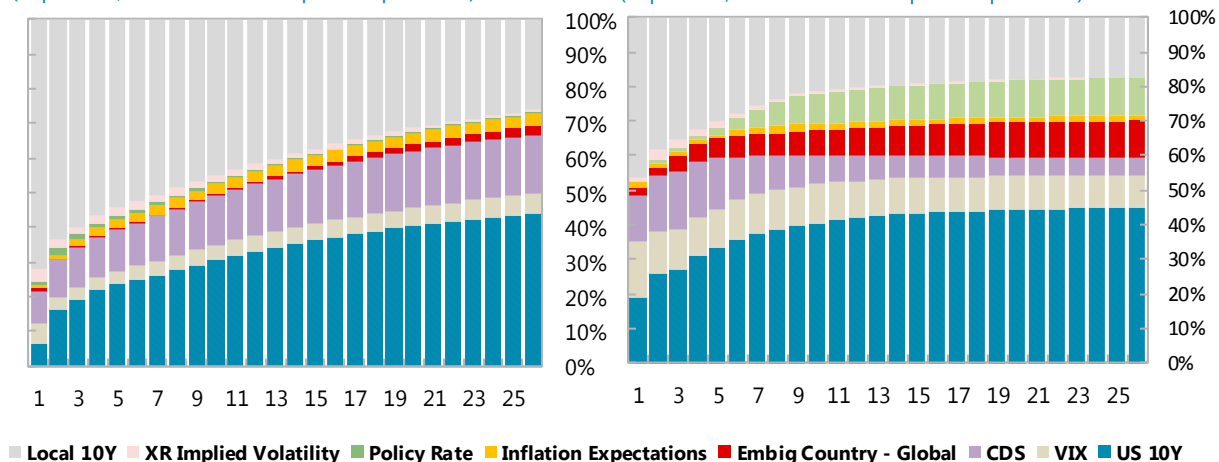
Variance decomposition of Brazilian Local 10Y bonds (in percent, cumulative decomposition per week)
