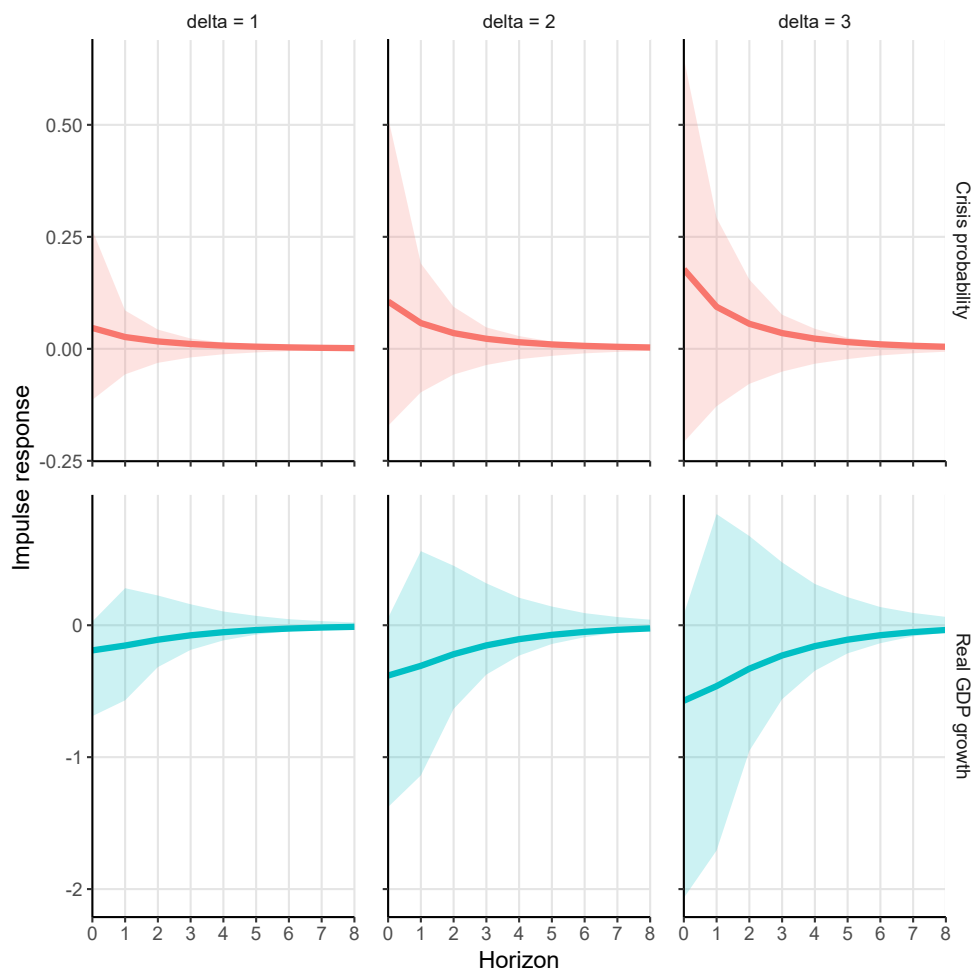
Figure C.5: GIRF analysis of a borrower macroprudential tightening: Advanced Economies
