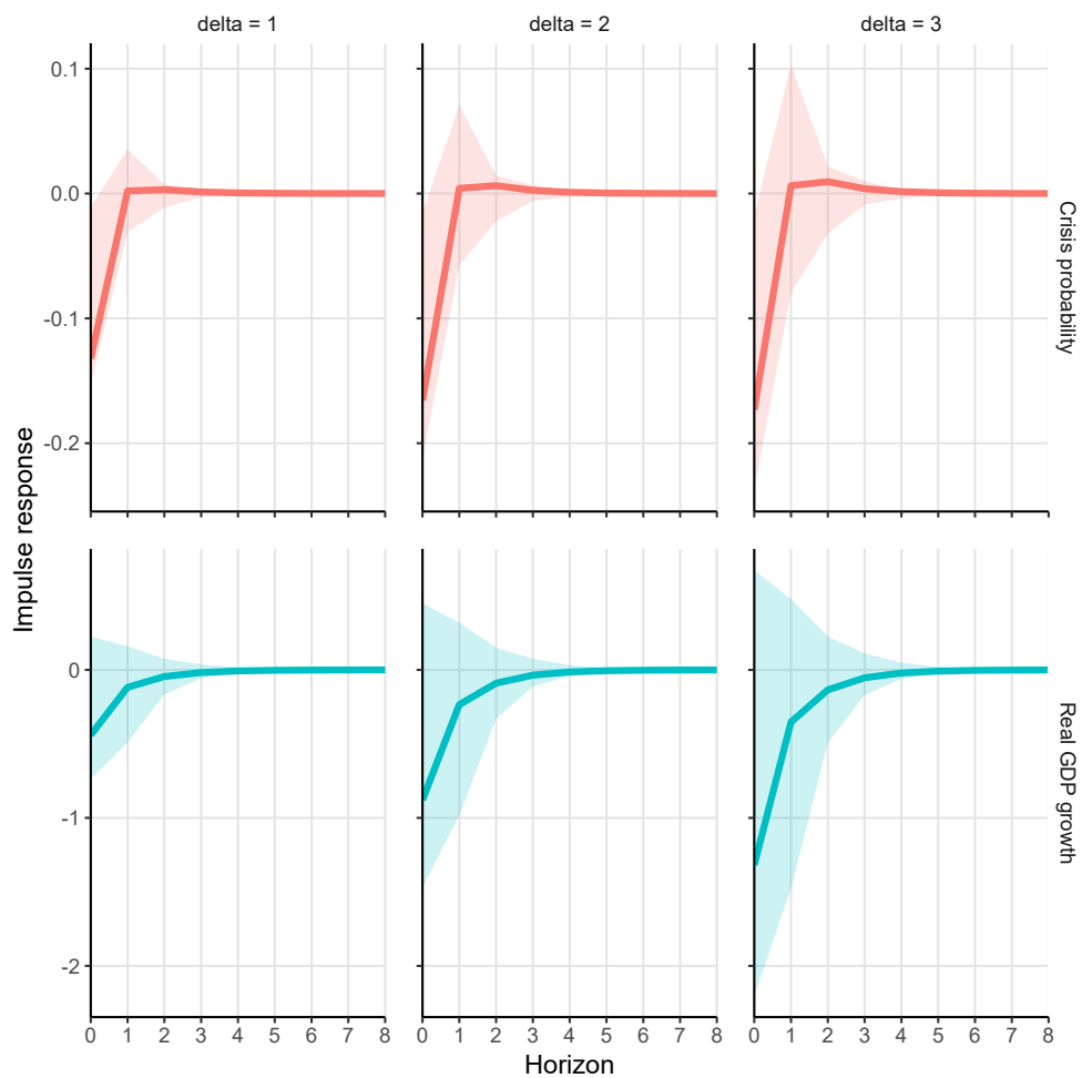
Figure C.6: GIRF analysis of a borrower macroprudential tightening: Emerging Market Economies
