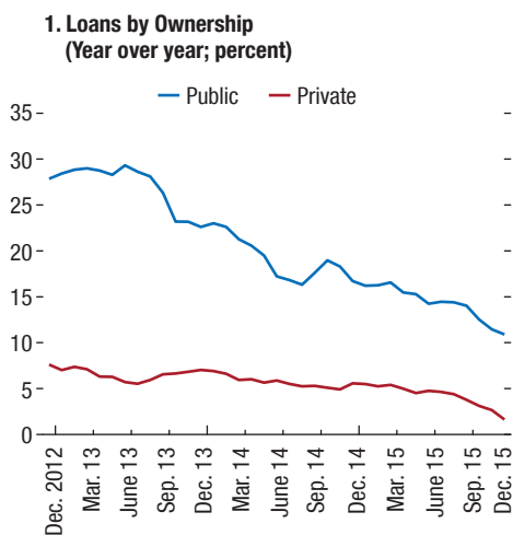
Figure 1.2.2. Performance of the Banking System in Brazil
