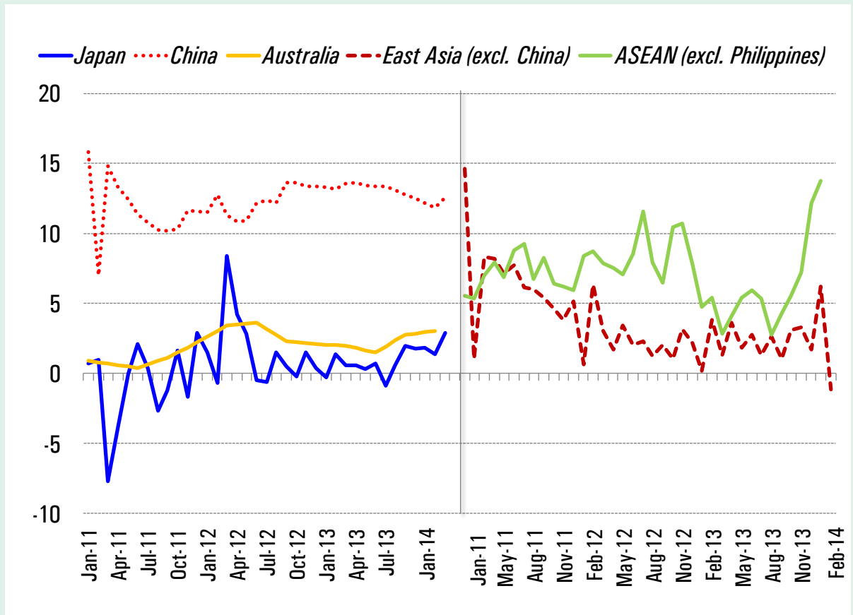
Figure 1.8. Selected Asia: Retail Sales Volumes
